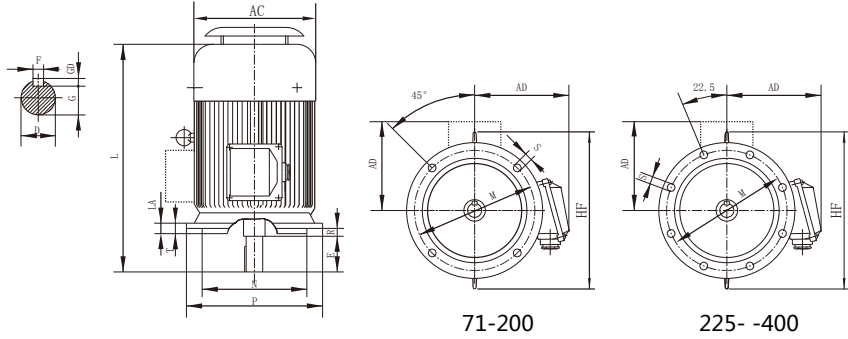
V1安装型式尺寸 DIMENS FOR MOUNTING ARRANGEMENTS V1
