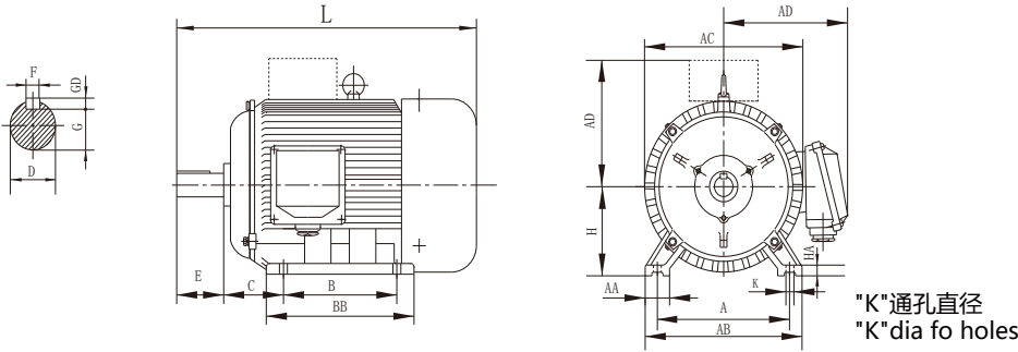
B3安装型式尺寸DIMENSIONS FOR MOUNTING ARRANGEMENTS B3
