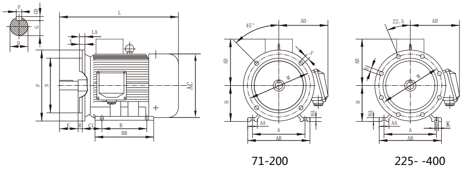
B35安装型式尺寸 DIMENSIONS FOR MONTING ARRANENTS B35
