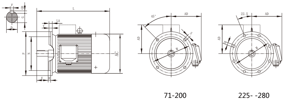
B5安装型式尺寸 DIMENSIONS FOR MOUNTING ARRANGEMENTS B5
